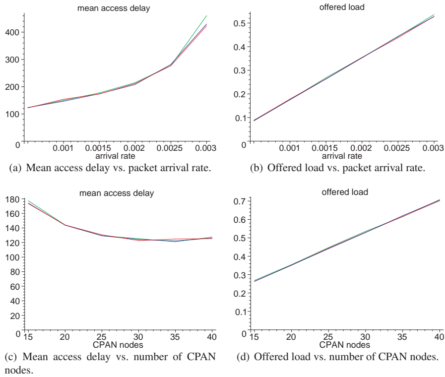
Fig. 11 Adaptive protocol: data transmission performance.
