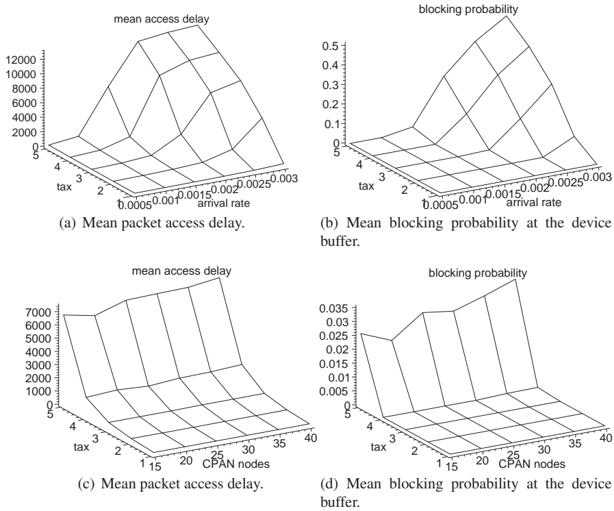
Fig. 10 Protocol modified to include local selection of the channel to sense: data communication performance. Top row: variable packet arrival rate and tax coefficient; bottom row: variable number of CPAN nodes and tax coefficient.
