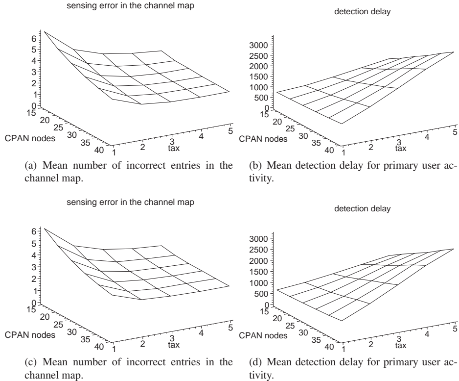
Fig. 9 Sensing performance of the protocol modified to account for least recently sensed channels, part II: local selection of channels to sense.
