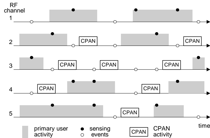
Fig. 1 Frequency hopping in a CPAN.
