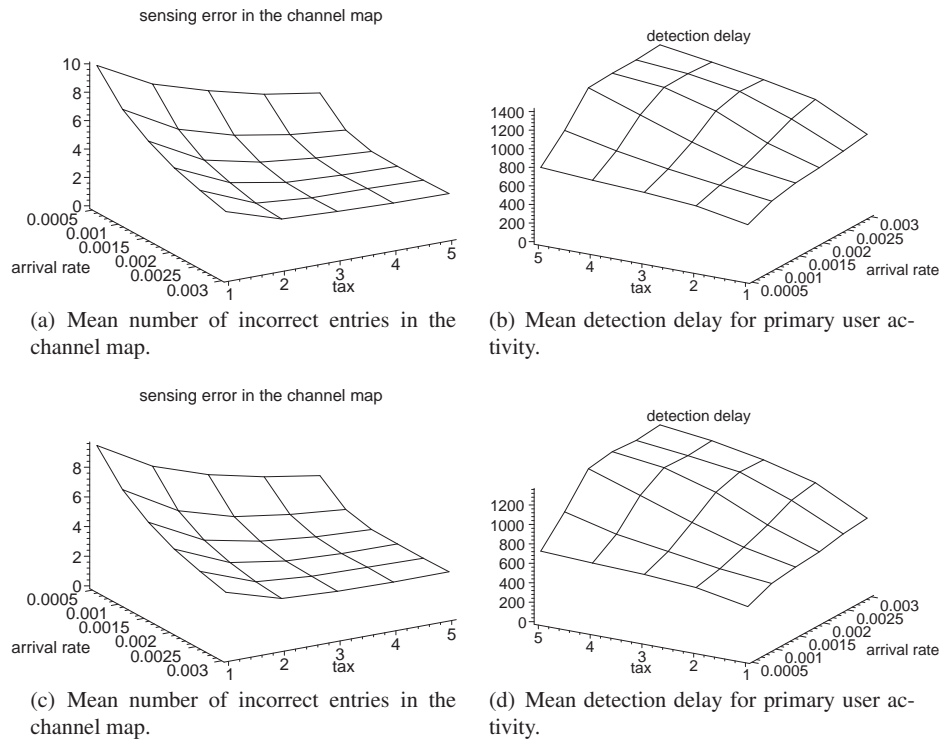
Fig. 8 Sensing performance of the protocol modified to account for least recently sensed channels, part I: centralized selection of channels to sense.
