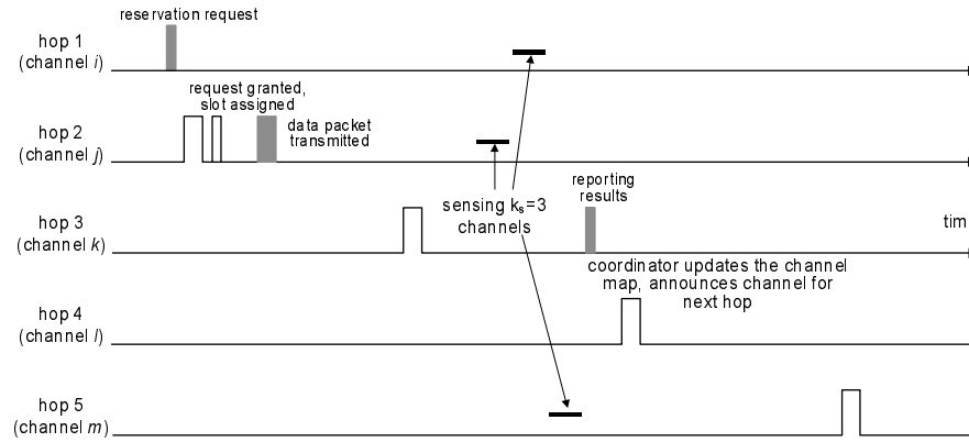
Fig. 2 CPAN operation: node activity for a single data packet to be transmitted.
