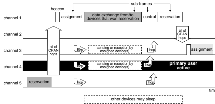
Fig. 3 Superframe format and node activities.
