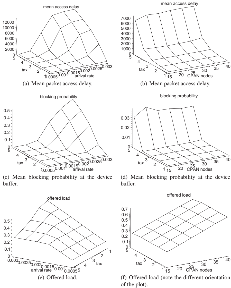
Fig. 5 Original transmission tax protocol: data communication performance. On the left, variable packet arrival rate and tax coefficient; on the right, variable number of CPAN nodes and tax coefficient.
