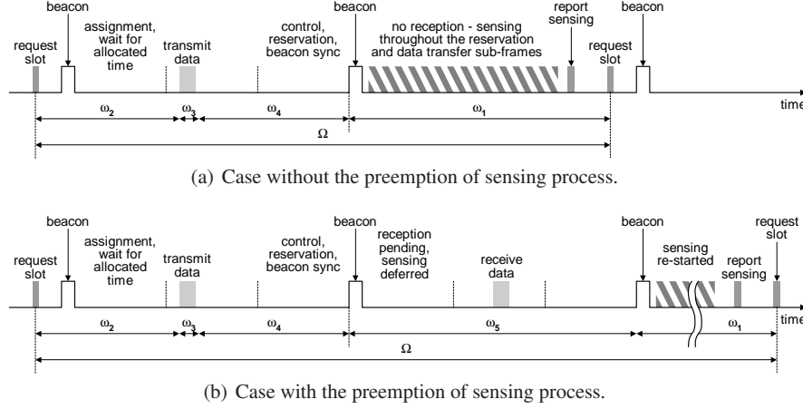
Fig. 4 Timing of node operation and distribution of arrivals during a service cycle.
