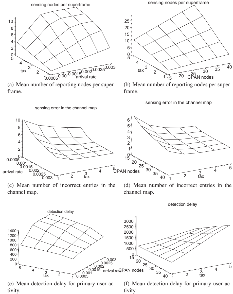
Fig. 6 Original transmission tax protocol: sensing performance. On the left, variable packet arrival rate and tax coefficient; on the right, variable number of CPAN nodes and tax coefficient.
